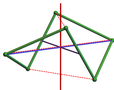
twist D_2 (4)
