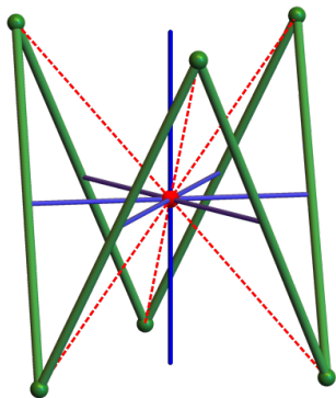
crown D_{3d} (12)
