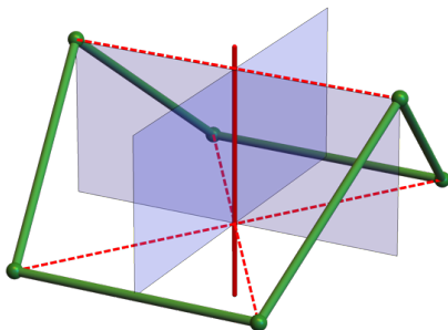
boat C_{2v} (4)
