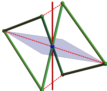
cross C_{2h} (4)
